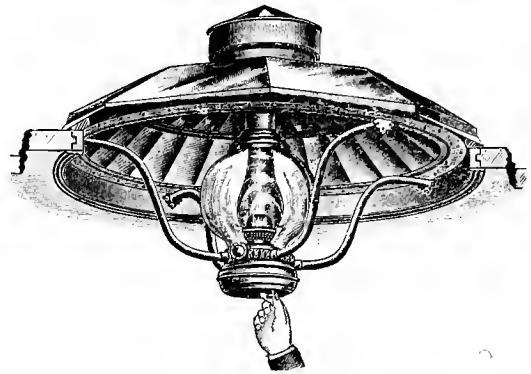
Fig. 3309. STREET-CAR CENTER-LAMP. Spread of arms, 25 ins. Drop, 12 3/4 ins.
